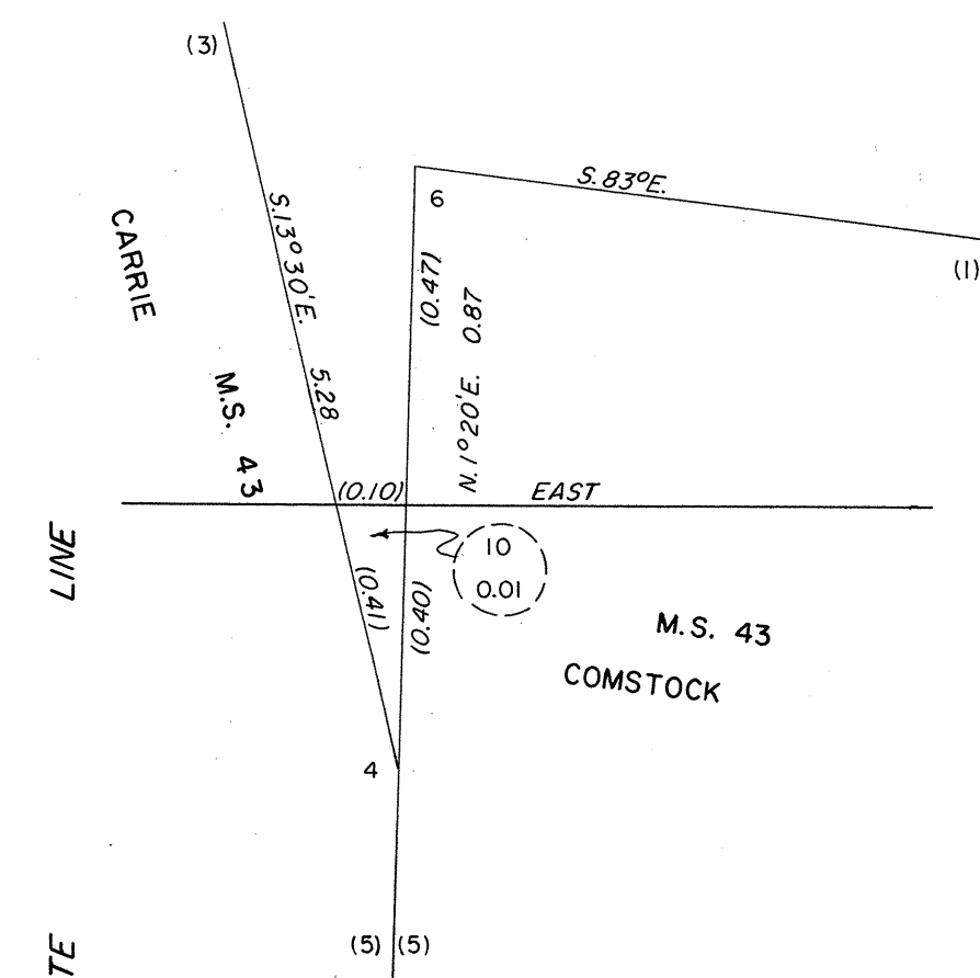
ENLARGED DIAGRAM
