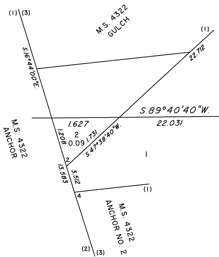
DETAIL "M" Not to Scale
