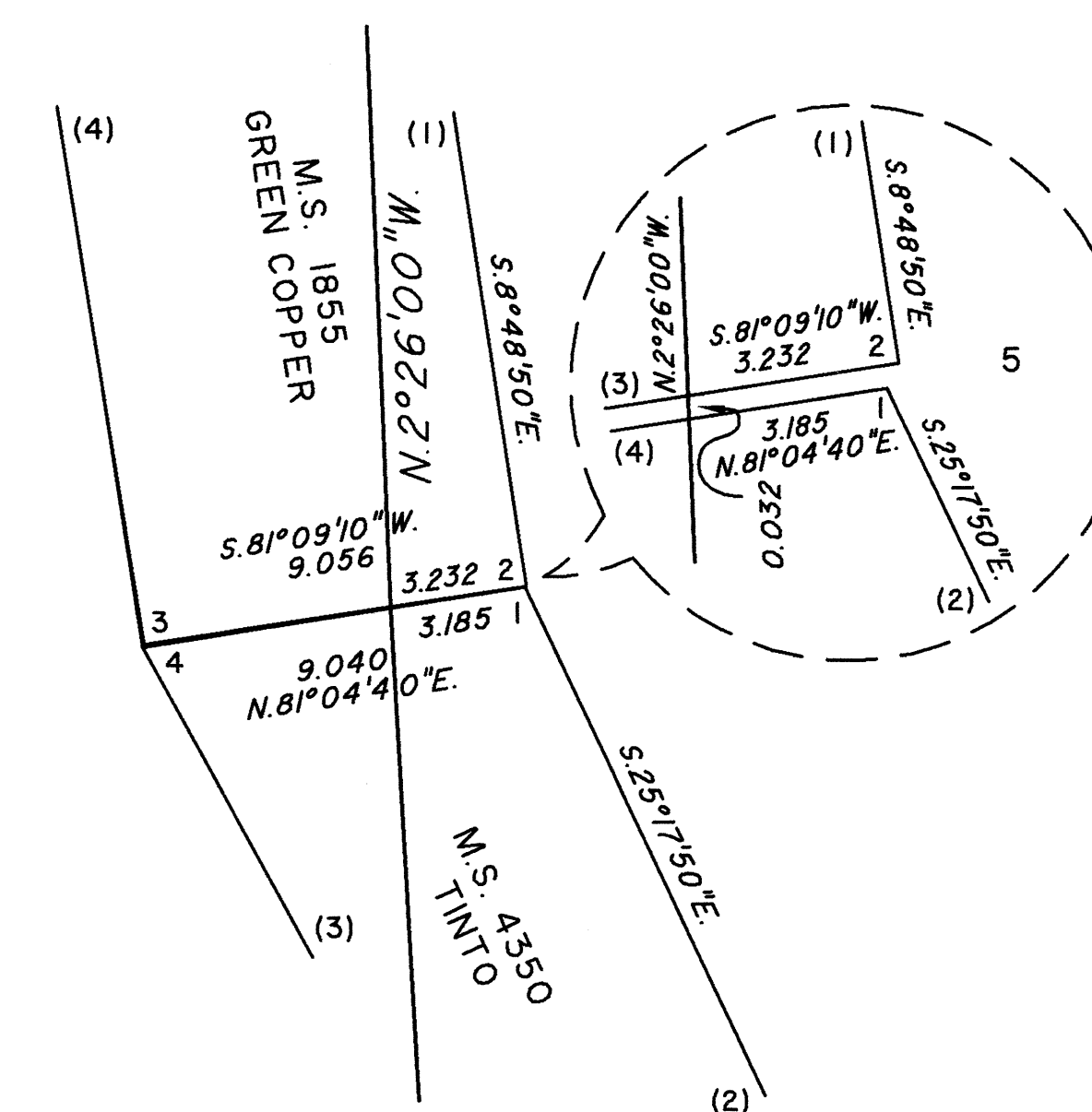
DETAIL "H" Not to Scale
