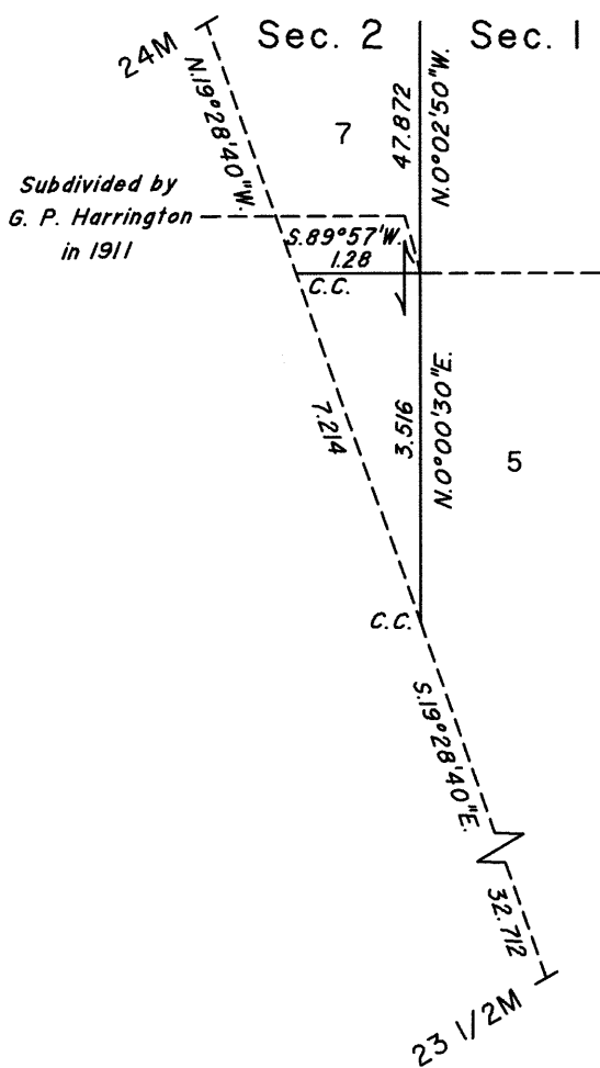
DETAIL "B" Not to Scale
