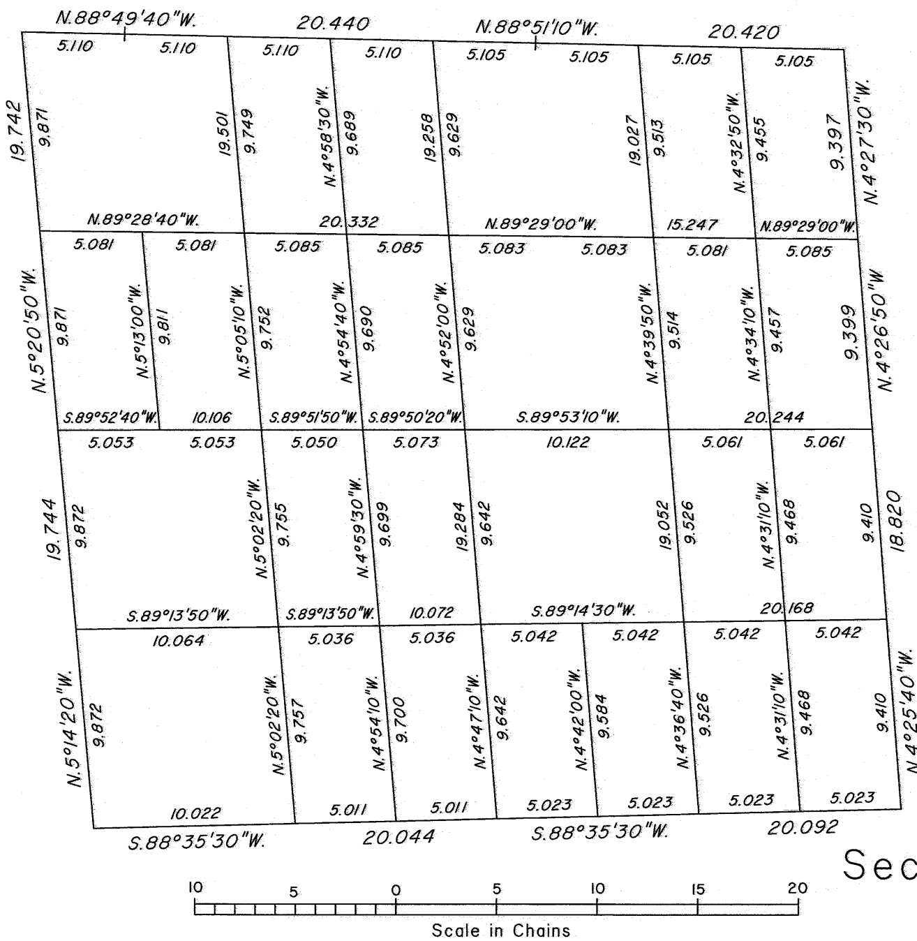
ENLARGED DIAGRAM NW1/4
