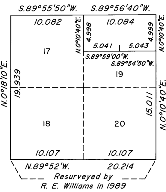
DETAIL "D" Not to Scale
