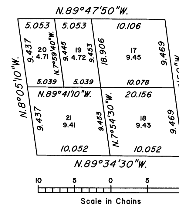
ENLARGED DIAGRAM NE1/4 SW1/4 Sec. 32
