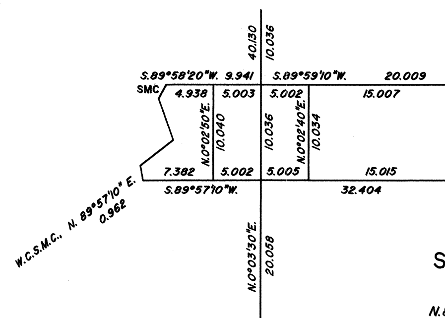
Detail C Sec. 14 Not to Scale
