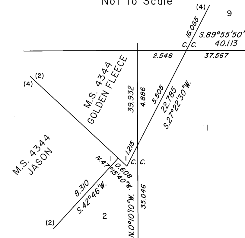
DETAIL "B" Not to Scale
