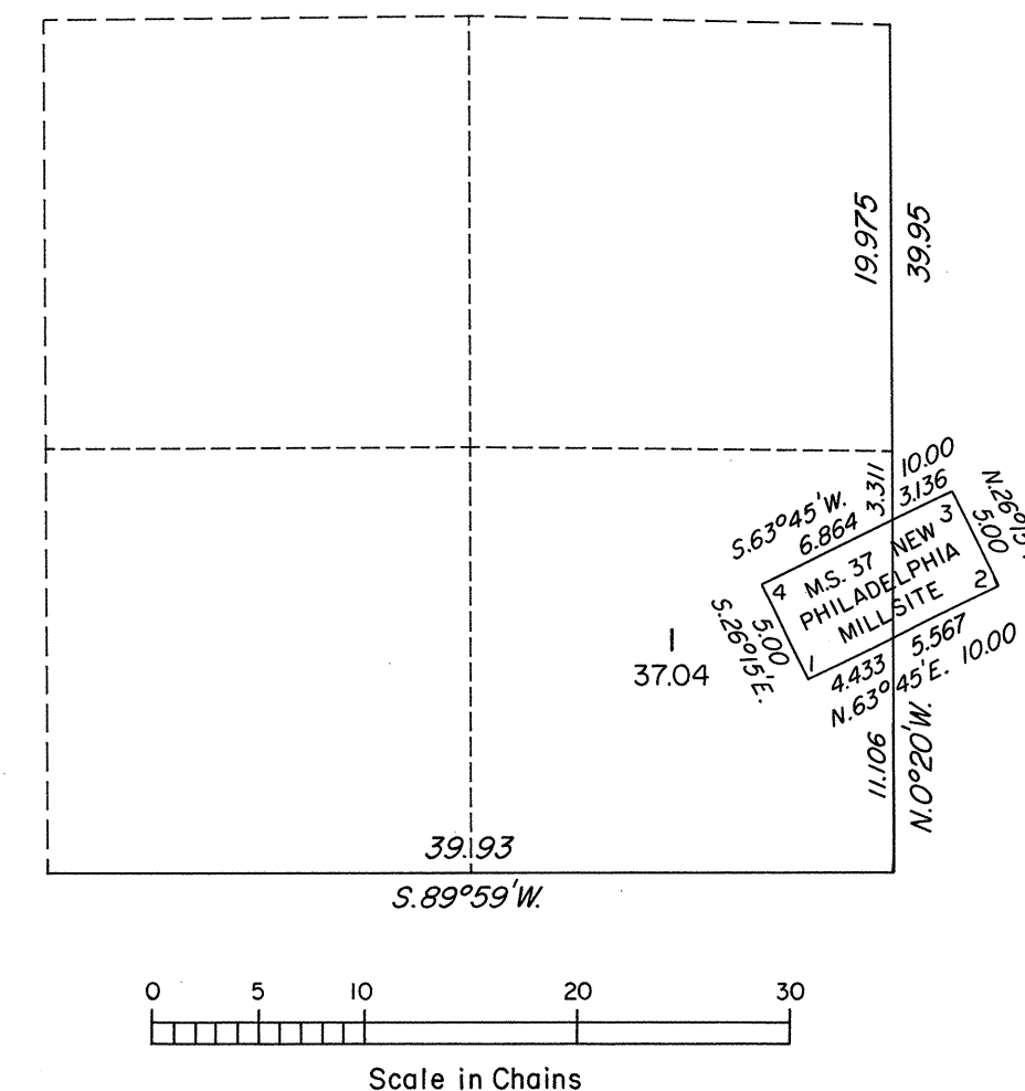
ENLARGED DIAGRAM OF THE SE 1/4 OF SECTION 33
