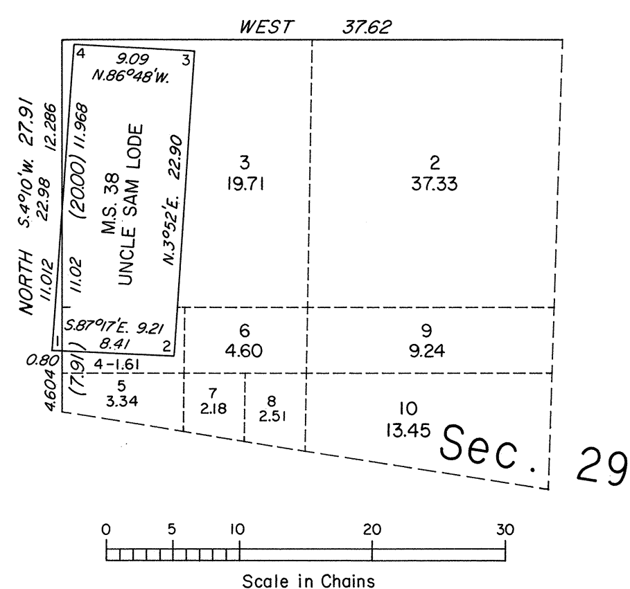
ENLARGED DIAGRAM OF THE NW 1/4 OF SECTION 29
